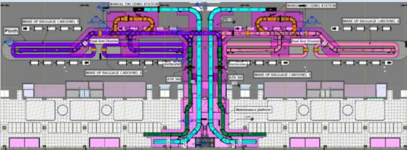
JED BHS Project – APR 2024 to DEC 2025 ST Sortation Zone
